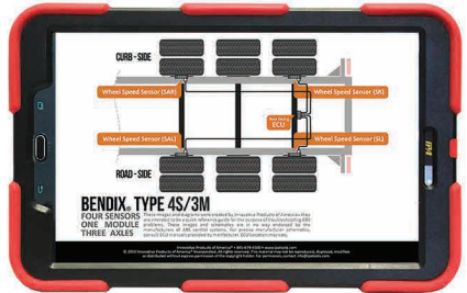
Base Functions Work with or Without Tablet
